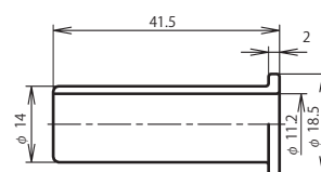
Cable bushing : NET-24-CB
