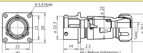
NAW-20 ■ -Ad(F)M □
