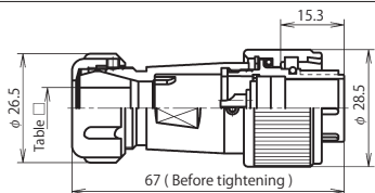
NAW-20 ■ -PF □
