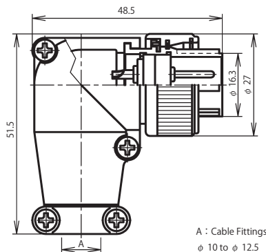
NR-20 ■ -LPM
