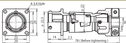
NAW-20 ■ -Ad(F)MK □
