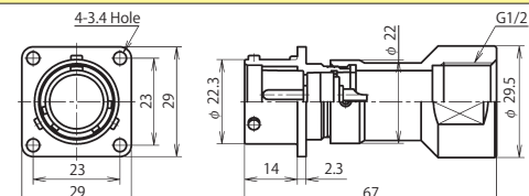
NAW-20 ■ -GAd(F)M1/2 ( Note )
