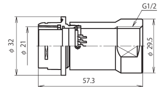
NR-24 ■ -GAdF1/2 ( Note )
