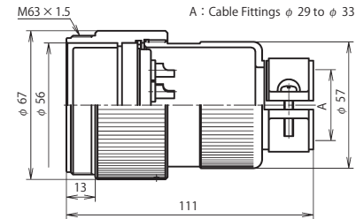
NCS-60 ■ -AdF
