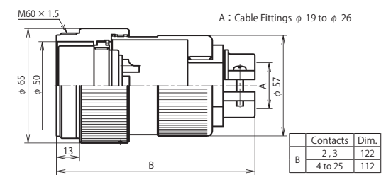
NCS-54 ■ -AdF
